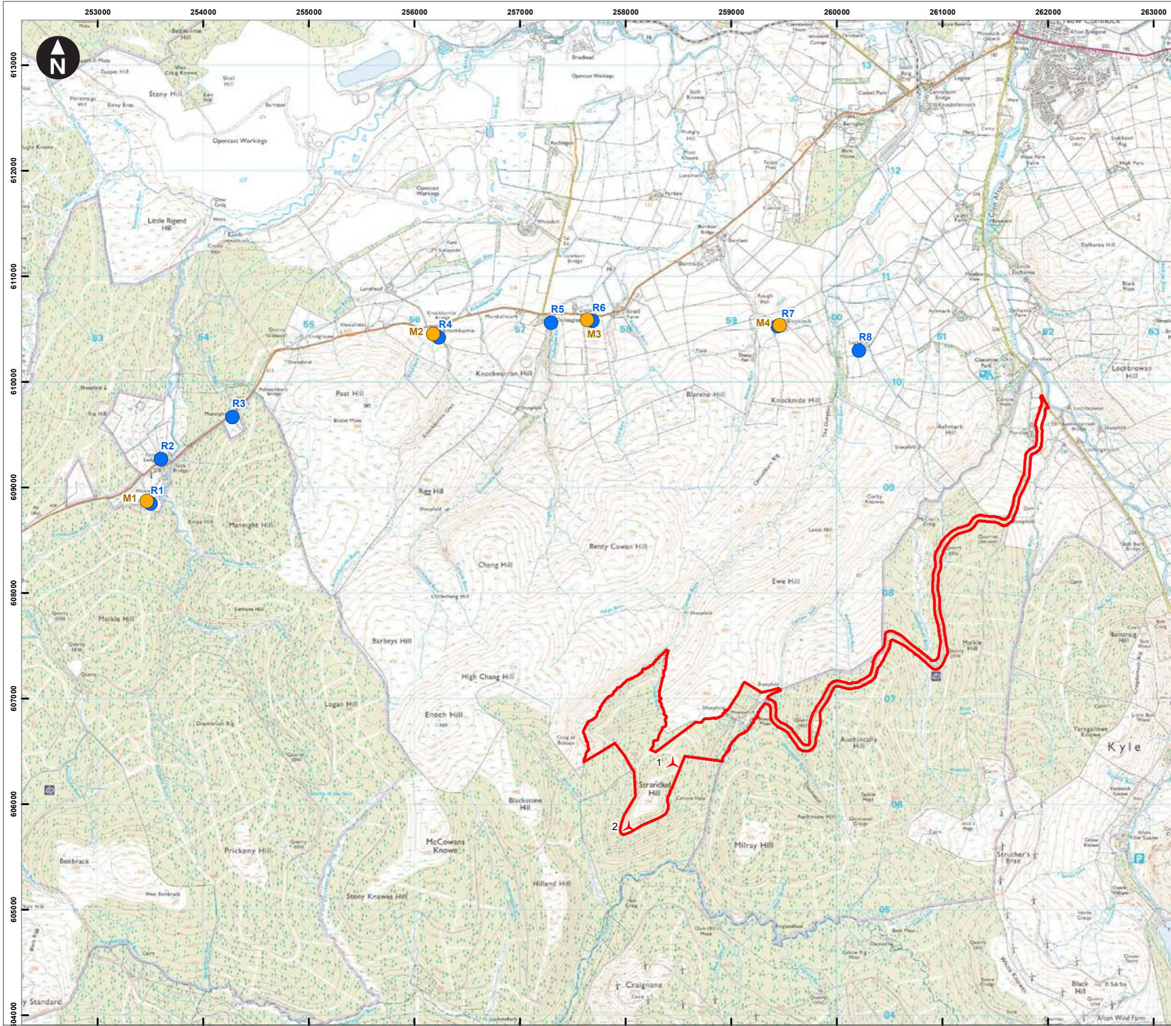
Figure 7.1 Assessed noise sensitive receptors and noise monitoring locations (2013 survey)
