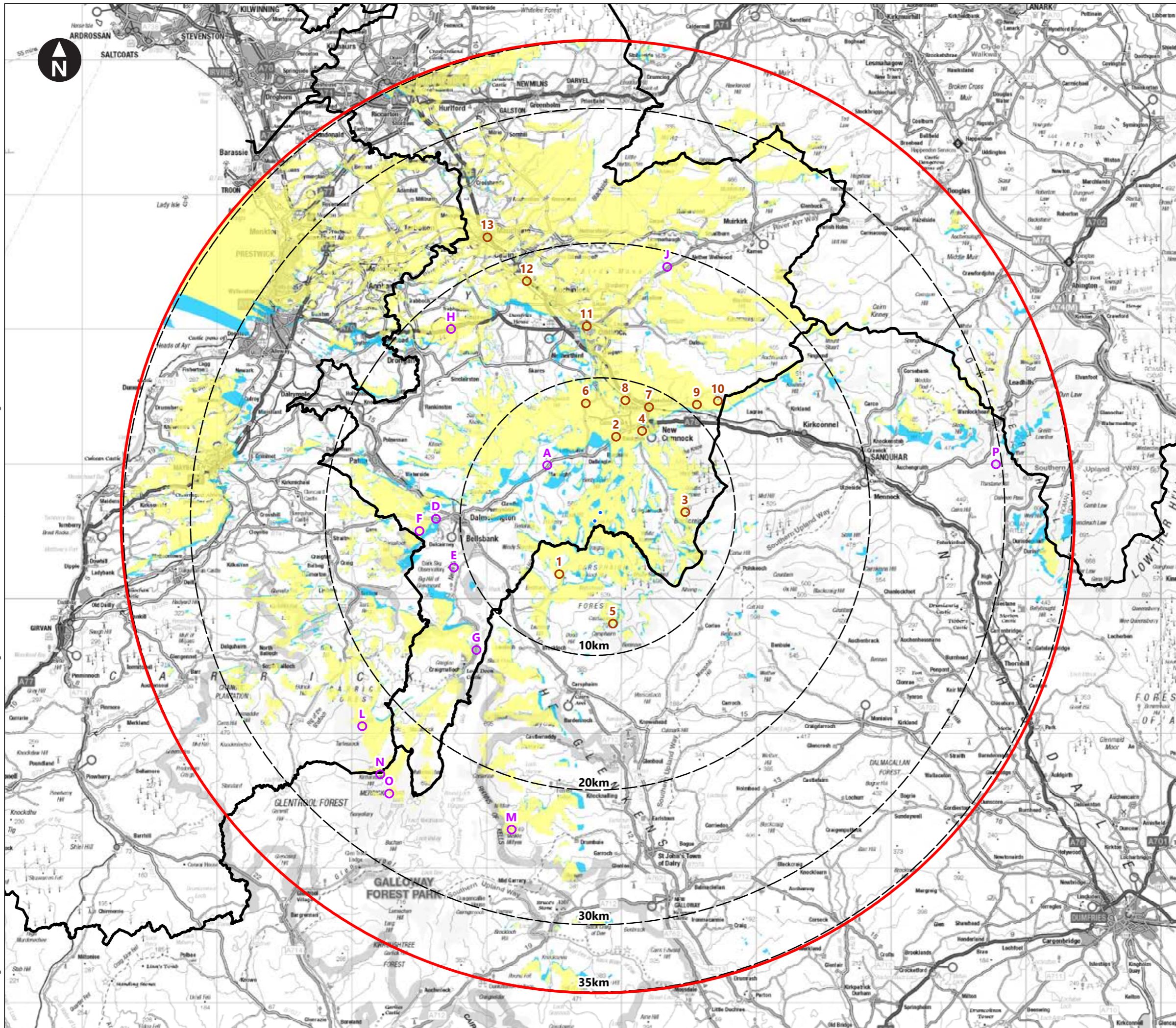
Figure 9.2 Zone of Theoretical Visibility (ZTV) to Blade Tip with Viewpoints
